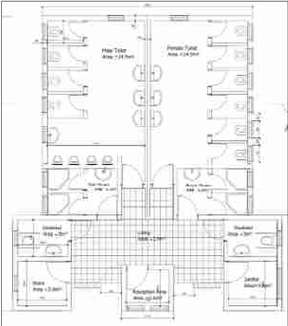
Figure 6: Floor Plan for Public Toilet
